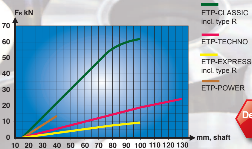
Radial force – shaft size.
